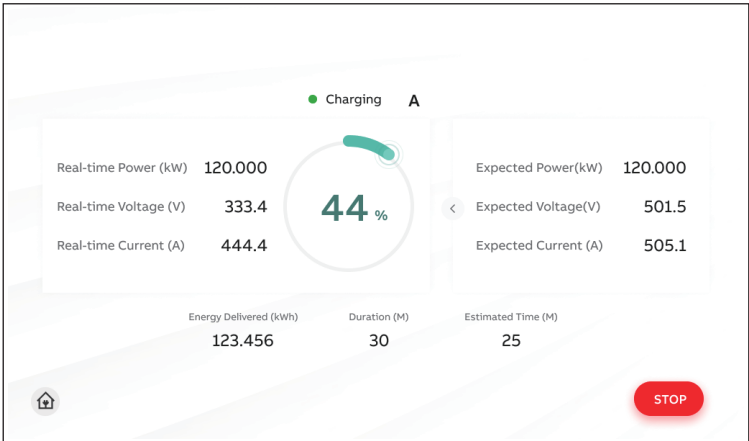
The display shows the detailed charging data for single charging gun.
